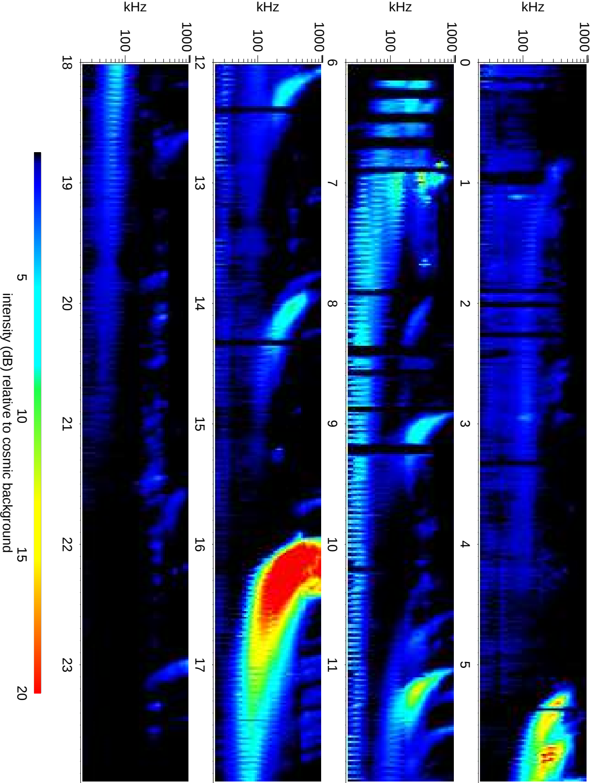
Wind Waves RAD1 receiver: 2014/07/30
