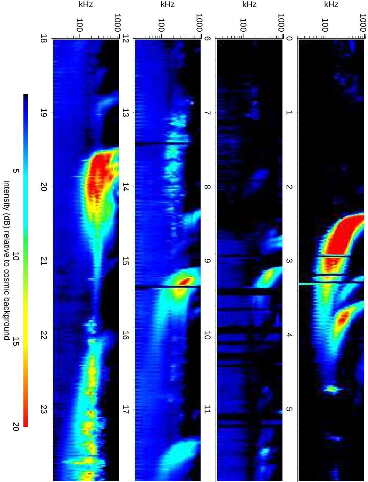
Wind Waves RAD1 receiver: 2014/01/17
