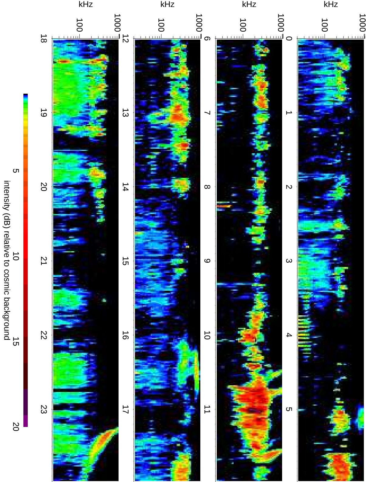
Wind Waves RAD1 receiver: 2007/01/21
