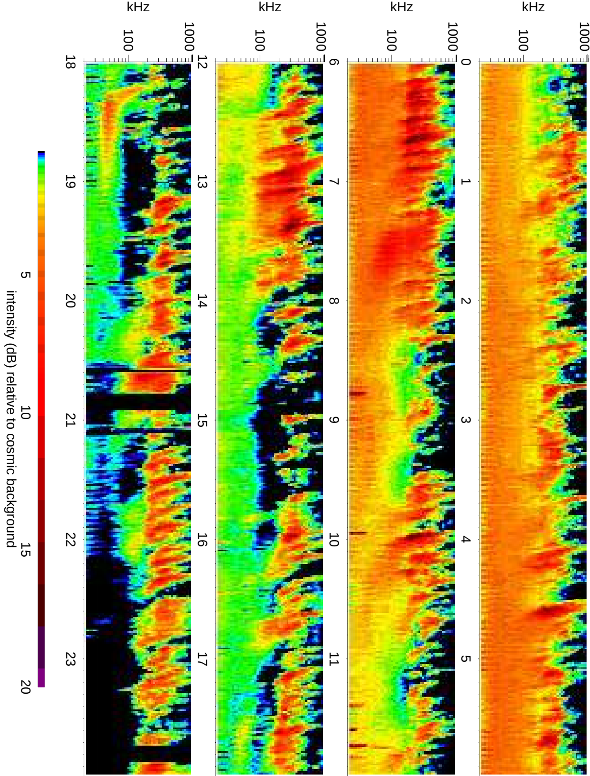
Wind Waves RAD1 receiver: 2007/01/11
