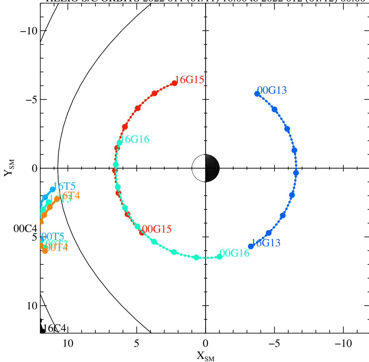
HELIO S/C ORBITS 2022 011 (01/11) 16:00 to 2022 012 (01/12) 00:00
