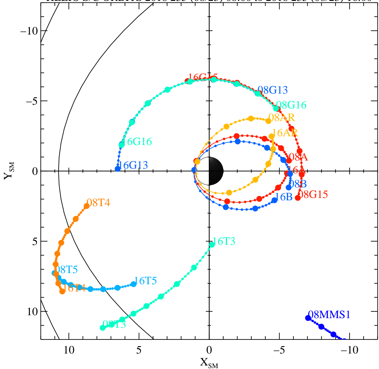
HELIO S/C ORBITS 2018 235 (08/23) 08:00 to 2018 235 (08/23) 16:00
