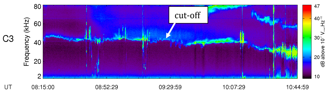
Figure 13: Example of a Natural spectrogram obtained on C3 on January 15, 2007, showing a clear natural cut-off in the Solar Wind.
