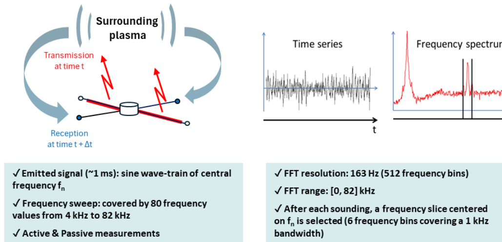
Figure 1: WHISPER instrument schematic operation in Sounding mode. Left panel shows the measurement principle. Right panel shows the on-board processing chain of the received signal and selection of a part of the power spectrum.
