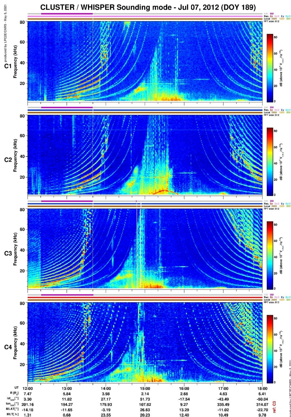
Figure 14: Example of a CSA WHISPER quicklook in Sounding mode, showing spectrograms of electric spectral power density for the 4 spacecraft, as well as technical parameters (colour bars).
