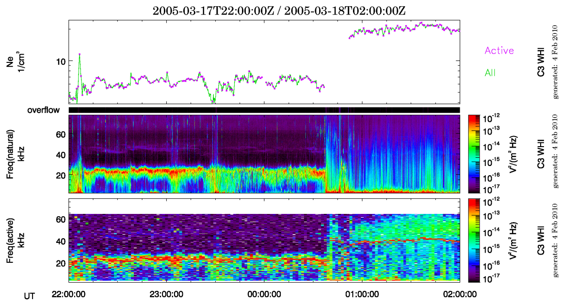
Figure 18: Example of density values and Natural and Active spectrograms (from top to bottom) for C3 on March 17, 2005, corresponding to solar wind/magnetosheath transition. Density values extracted from the Active WHISPER spectra are plotted as purple points whereas green line represents the density extracted from both Active and Natural measurements.
