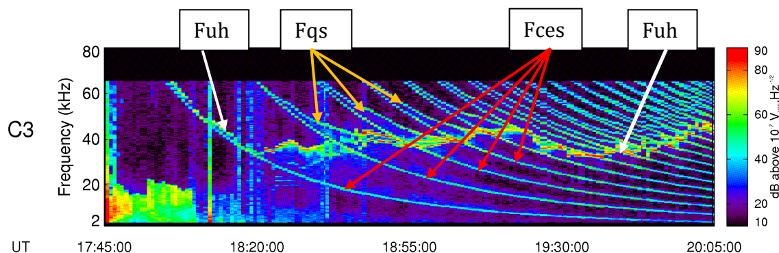
Figure 12: Example of an ACTIVE spectrogram obtained on C3 on January 30, 2009, showing resonances excited at the outward leg of the plasmasphere.
