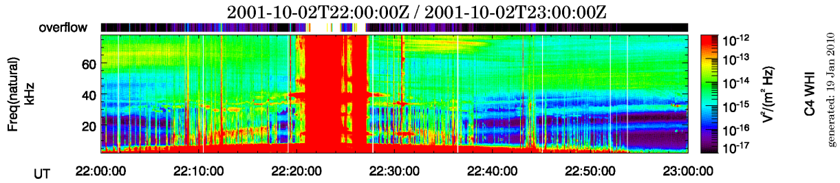
Figure 6: Example of a WHISPER electric spectral power density spectrogram affected by overflows on C4 for October 02, 2001, around 22:25 UT. The upper bar gives the colour-coded overflow rate.
