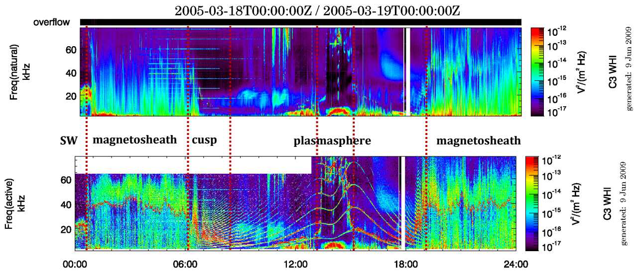
Figure 2: Spectrograms acquired in Natural mode (top) and Sounding mode (bottom) on C3, March 18, 2005 showing several typical magnetospheric signatures of solar wind (SW), magnetosheath, cusp, and plasmasphere.
