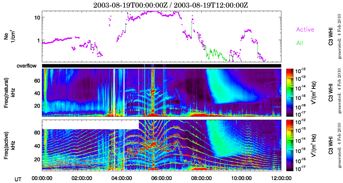
Figure 17: Example of density values and Natural and Active spectrograms (from top to bottom) for C3 on August 19, 2003, corresponding to a plasmasphere crossing. Density values extracted from the Active WHISPER spectra are plotted as purple points whereas green line represents the density extracted from both Active and Natural measurements.
