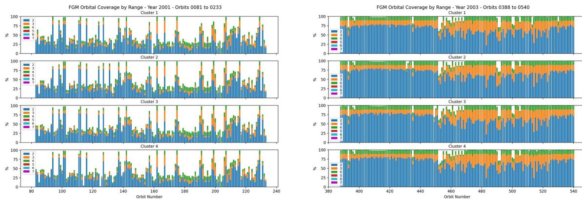
Figure 7, FGM data coverage as a fraction of the orbital duration, 2001 (left) and 2003 (right); FGM range is colour-coded with ranges 2 (blue) and 3 (orange) constituting the majority of the measurement time.
