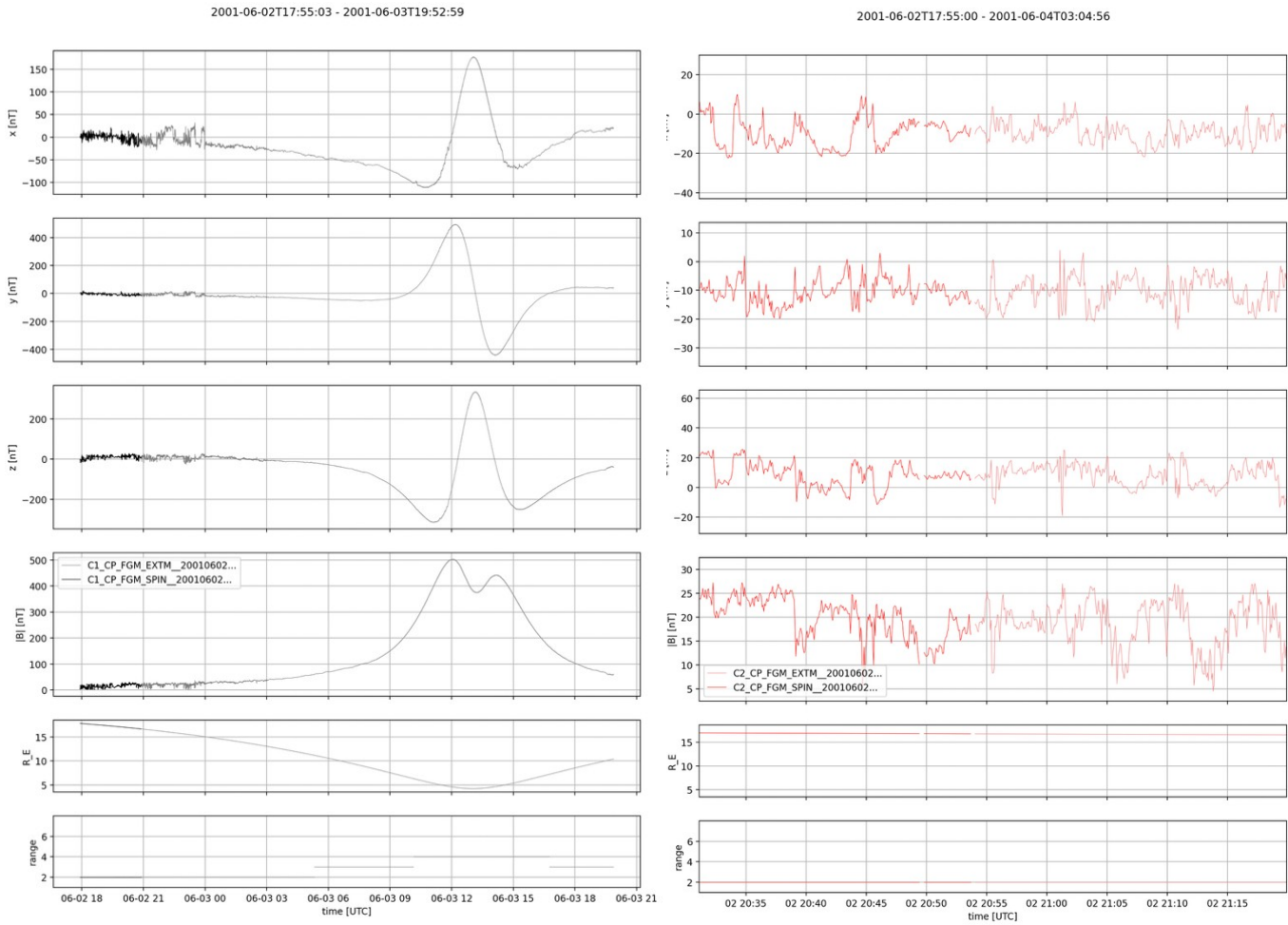
Figure 8, 2 nd June 2001 Extended Mode data (faint lines) compared with preceding archive SPIN data (heavy lines): left – Cluster 1, showing Extended Mode data completing the ‘no data-taking’ interval of 23 hours around perigee, right – Cluster 2, detail of the same interval showing the boundary between the Extended and regular SPIN data (Extended Mode starts at about 20:54 UTC in both cases)
