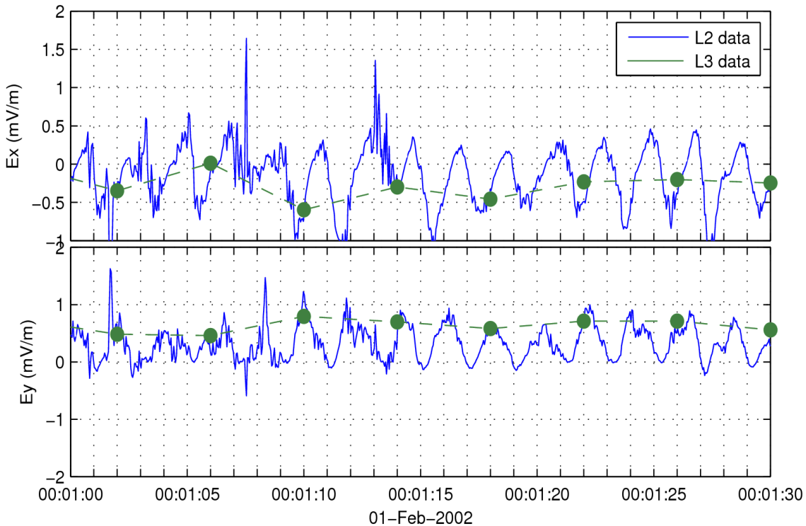
Figure 7: Comparison of L2 ( 25\text{ s}^{-1} , blue) and L3 (4 second resolution, green) for a period when only one probe pair was available.
