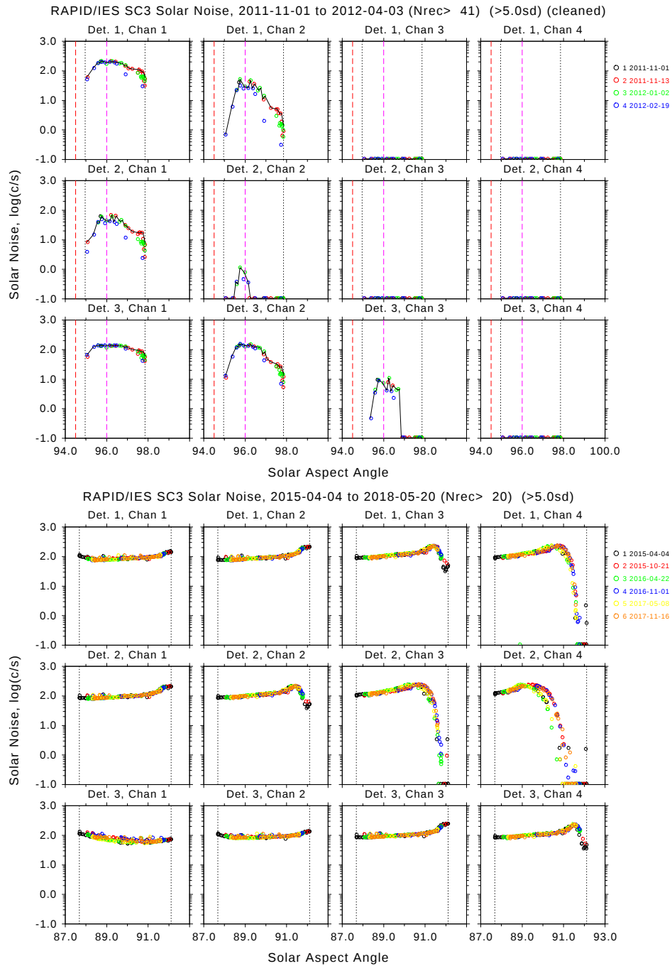
Figure 8: The dependence of the solar noise on SC3 with solar aspect angle (SAA). The plots show the noise for 3 detectors and 4 energy channels. The upper plot is from a time when the range of SAA on SC3 was shifted to accommodate RAPID (as well as could be done), while the lower plot shows data from 3 years after the space orientations were fixed and the SAA sweeps over the full range over one year. The different colours indicated different sweeps. It is clear that the dependence is reproducible over many sweeps, except for parts of detector 2, channel 4.
