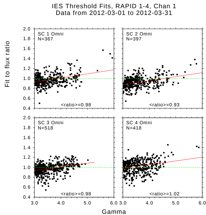
Figure 40: Ratio of extrapolated to measured flux in energy channel 1 after adding the energy defect. Data produced with IES calibration version V330.
