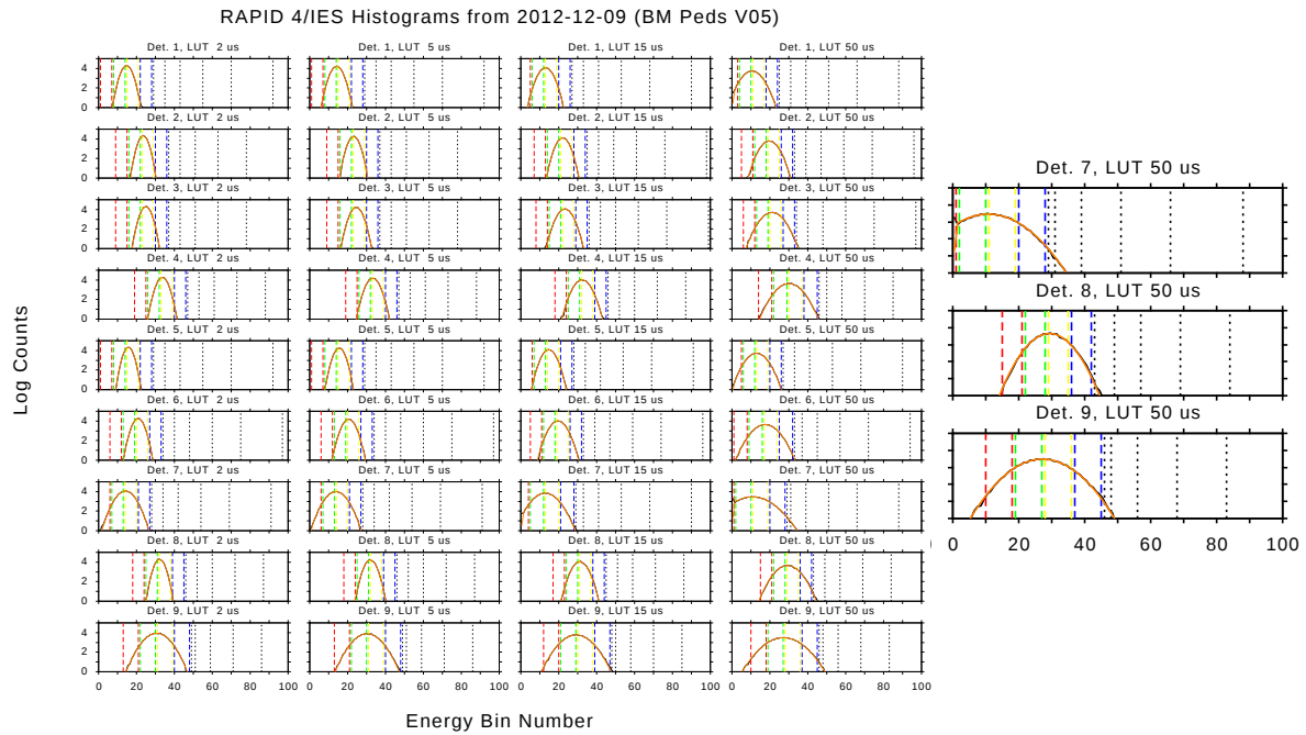
Figure 5: Histogram plots from SC4 on 2012-12-09, for each detector and integration time. The pedestal is especially broad for 50\ \mu\text{s} (right column) in detectors 7, 8, and 9 (see blow-up at right). The energy channel boundaries are indicated with black dashed lines. One sees how the pedestal extends to the first energy channel for detector 8, and even into the second one for detectors 7 and 9.
