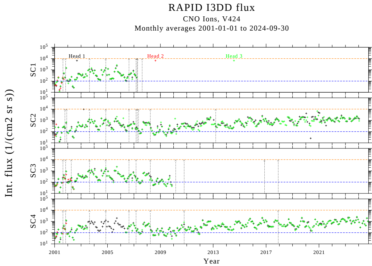
Figure 21: CNO fluxes from series 4 calibration, as in Figure 19
