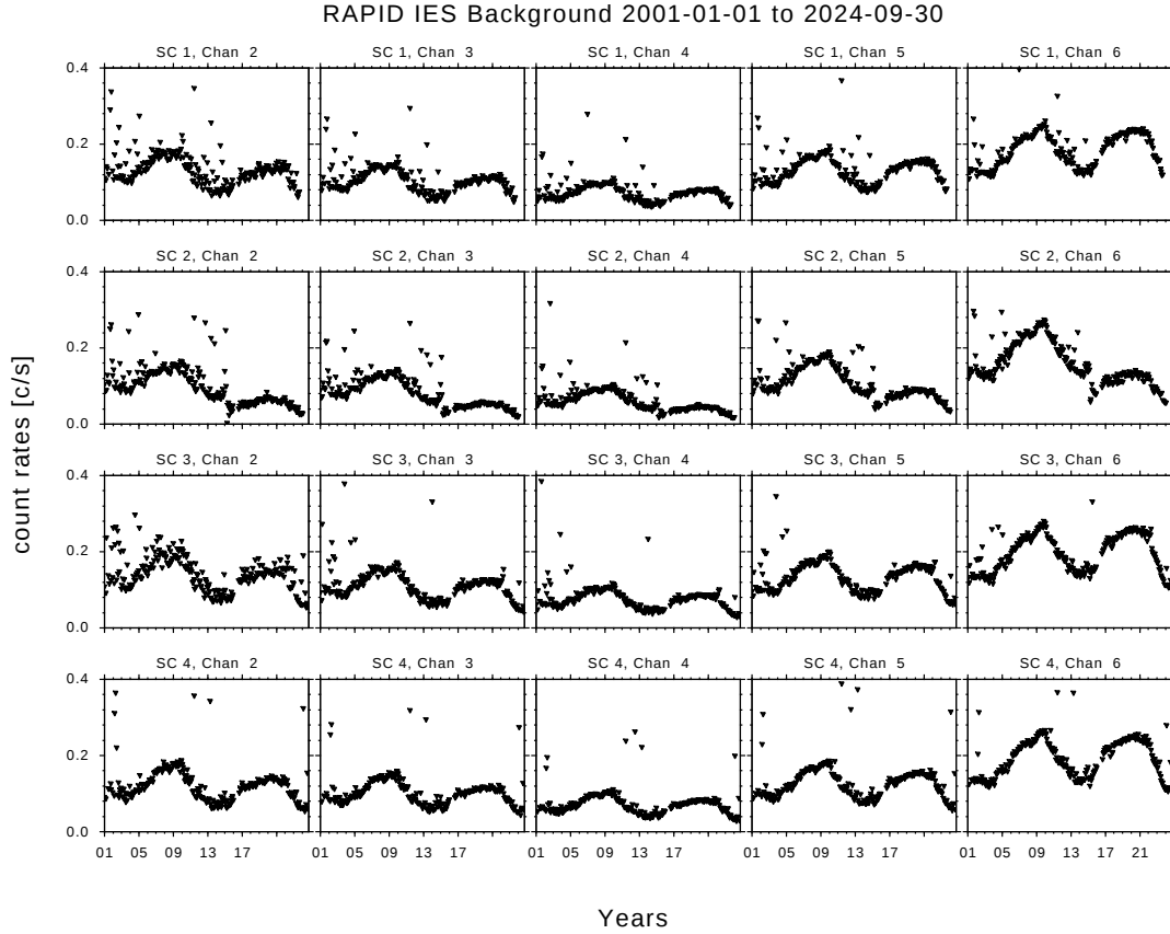
Figure 68: Minimum electron background rate per orbit over the entire mission of almost 24 years, for all 4 spacecraft and 5 energy channels. Channel 1 has been suppressed as described in the text. (The jump in the data on SC2 in 2015 is due to the partial failure in IES, Section 10).
