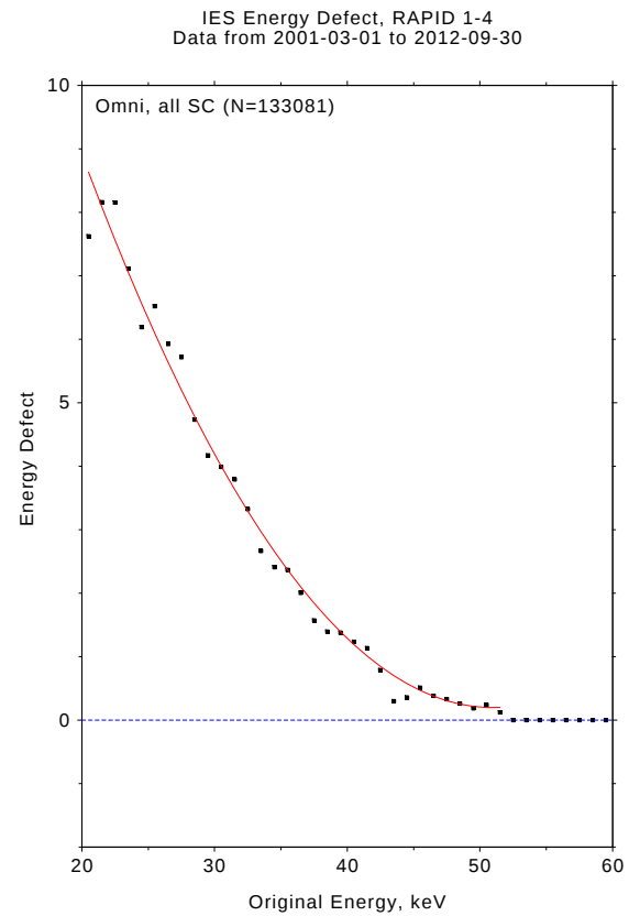
Figure 38: Energy defect plotted against original energy, for all spacecraft, all detectors, all modes, over 12 years from 2001 to 2012. The red curve is a quadratic fit to the defect values below 52 keV.
