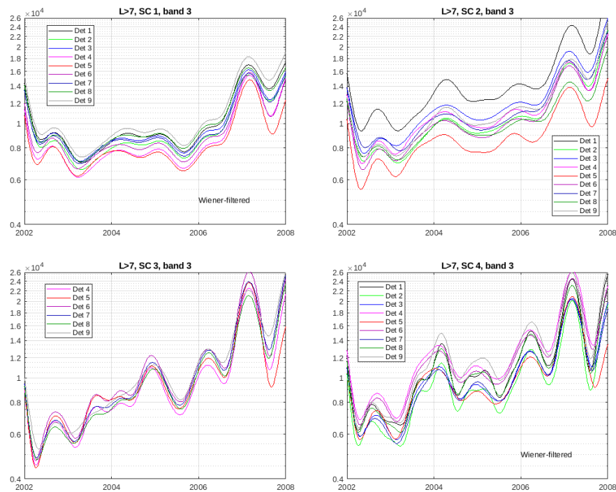
Figure 52: Uncorrected Wiener-filtered fluxes from median-filtered orbital averages (L>7) at energy channel 3 for the 9 detectors (polar directions) during the early mission. Note the scatter in the flux levels of the detectors especially on spacecraft 2 and the difference in the shape of the curves on spacecraft 4.
