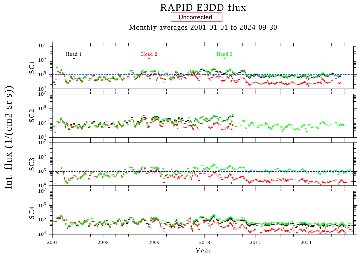
Figure 60: Uncorrected electron fluxes over the mission lifetime for all 4 spacecraft. Each point is a monthly average of the fluxes in each of the 3 detector heads, for L > 7 . The horizontal dashed line marks a certain level for comparison between the panels.
