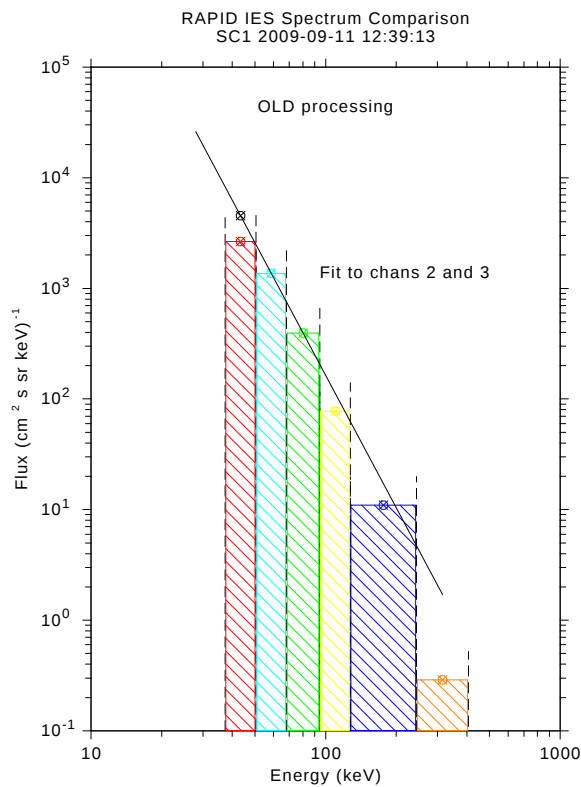
Figure 34: Example of the spectral analysis: a power law is fitted to channels 2 and 3, and then extrapolated back to the energy of channel 1 and compared to the measured flux.
