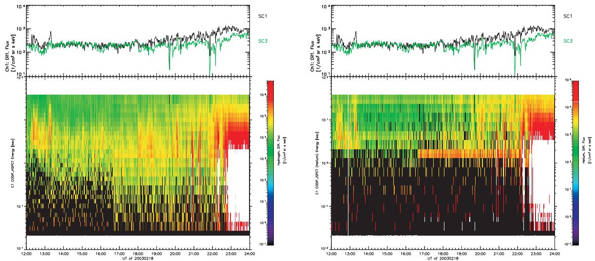
Figure 27: Energy spectrograms for CIS and RAPID proton (left) and helium (right) fluxes, 18 February, 2003.
