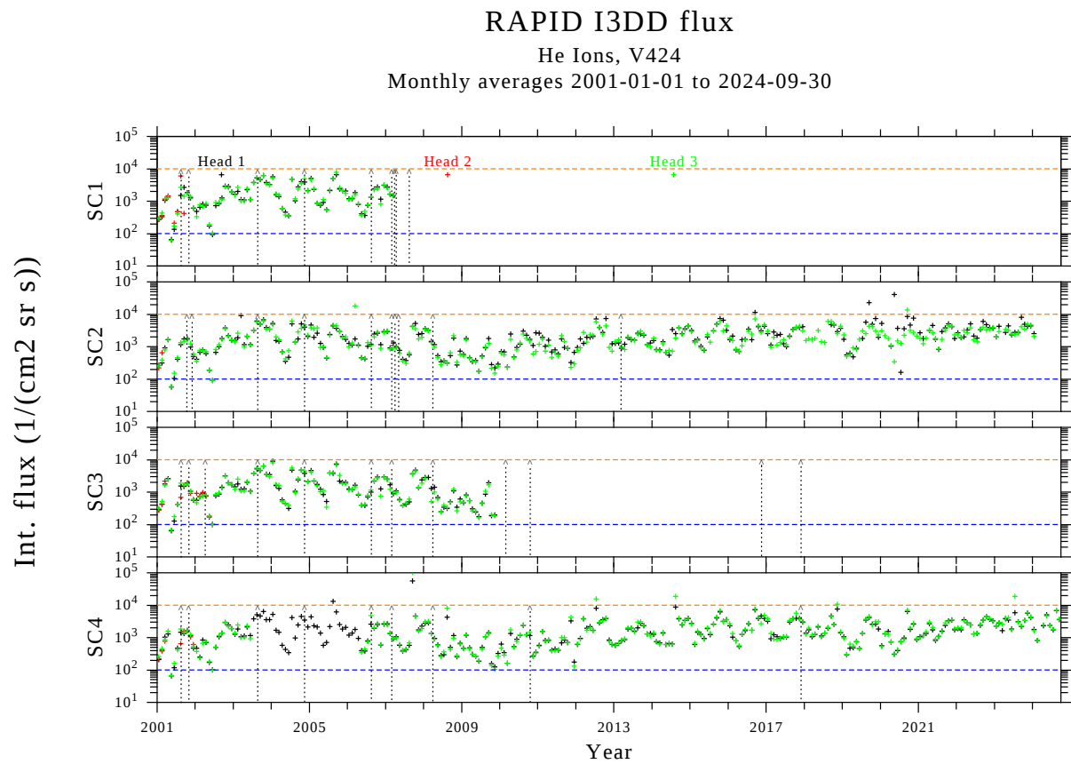
Figure 20: Helium fluxes from series 4 calibration, as in Figure 19.
