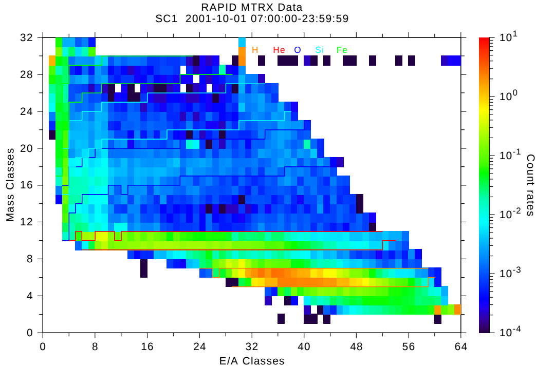
Figure 75: The MTRX space filled with data from 2001-10-01, the same interval as in Figure 73. The SRIM curves for the limiting incidence angles of 0^\circ and 30^\circ are also shown.
