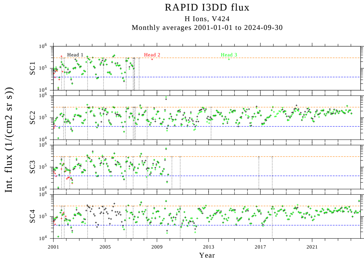
Figure 19: Hydrogen fluxes from series 4 calibration, in the same format as in Figure 16, i.e. monthly averages above 7 R_E .
