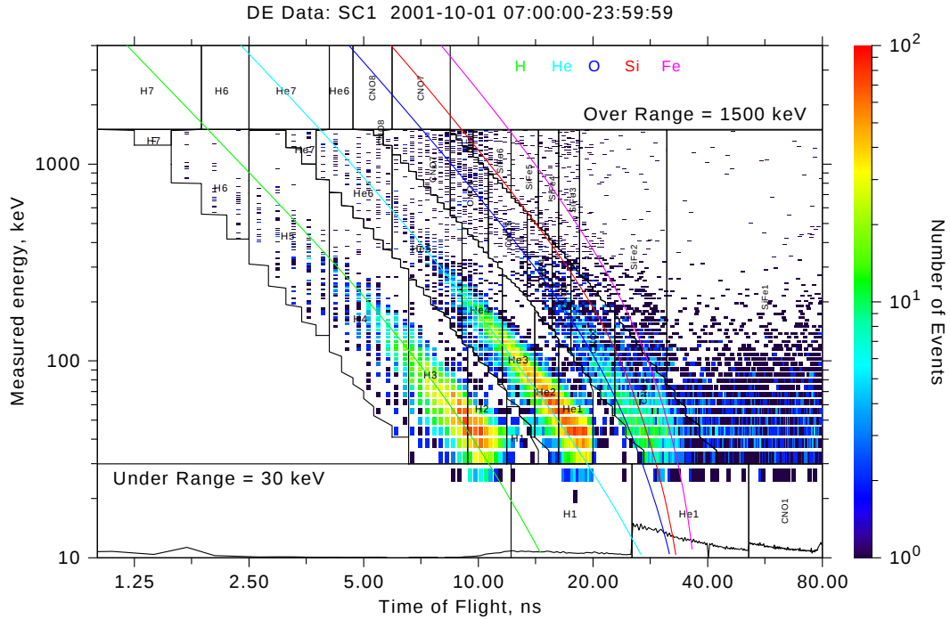
Figure 73: Direct Event space filled with data from 2001-10-01, during a very disturbed interval. Here one sees how well the H, He, and CNO fall in their expected areas, whereas other events line up reasonably well with the (SRIM) Fe line. There are even indications at higher energies of the possible presence of Si.
