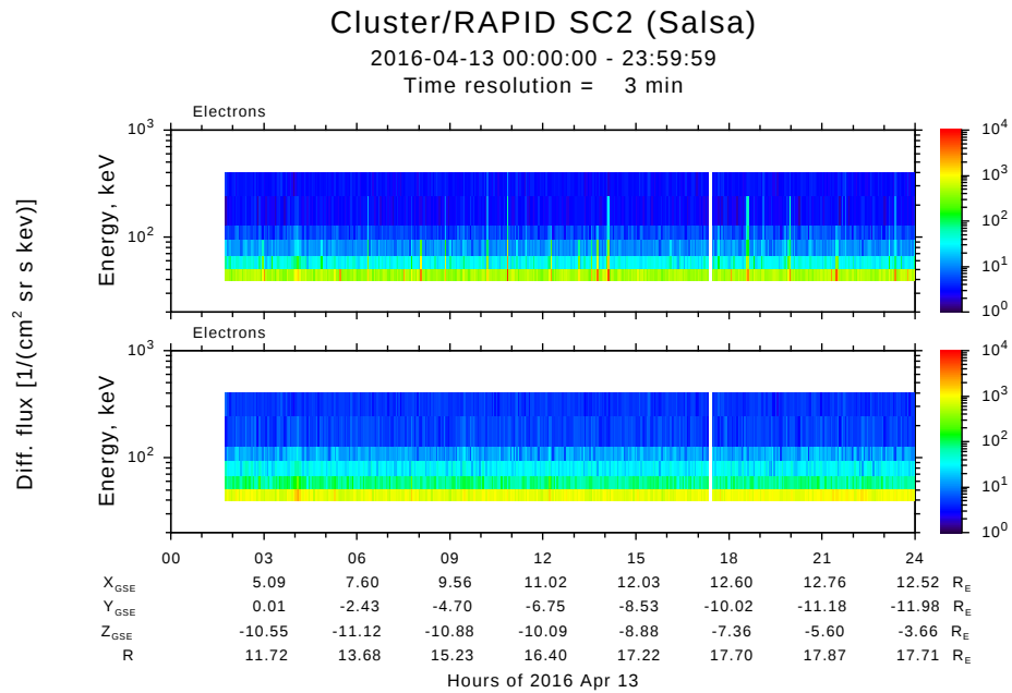
Figure 66: Additional noise spikes appear in the IES data after the partial recovery (upper panel) which can be detected and removed (lower panel).
