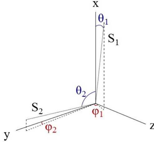
Figure 2: The relationship between the orthogonal (x,y,z) and sensor (S 1 ,S 2 ,S 3 ) coordinate systems. The angles \theta and \phi for each sensor coordinate are defined in the same way. The task of producing calibrated data then comes down to determining the parameters in this calibration equation. There are six angles, three gains and three offsets. There is no single calibration analysis that can be used to calculate all of these parameters. S 3 has been omitted for clarity. See [1] for more detail.
